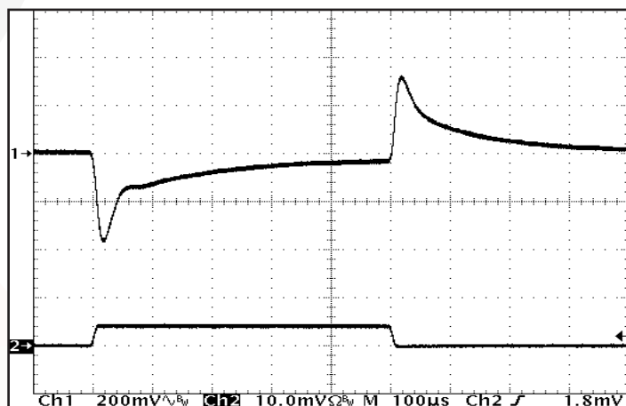
Figure 12: Output voltage response to step-change in load current 0%-50%-0% of I_{out} (max). Load cap: 1 \mu F ceramic cap and 10 \mu F, 100m \Omega ESR tantalum cap. Ch 1: Vout (200 mV/div). Ch 2: Iout (10 A/div).
