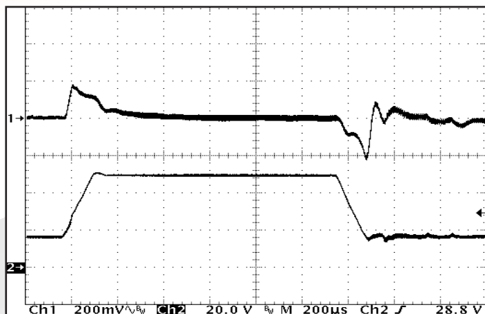
Figure 13: Output voltage response to step-change in input voltage (16 V - 50 V - 16 V). Load cap: 10μF, 100mΩ ESR tantalum cap and 1μF ceramic cap. Ch 1: Vout (200 mV/div). Ch 2: Vin (20 V/div).
