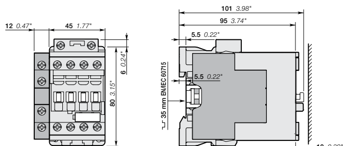
AF26, AF38 + CAL4-11 2-pole auxiliary contact block
