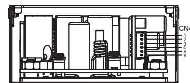
cross sectional view A Scale 1:1
