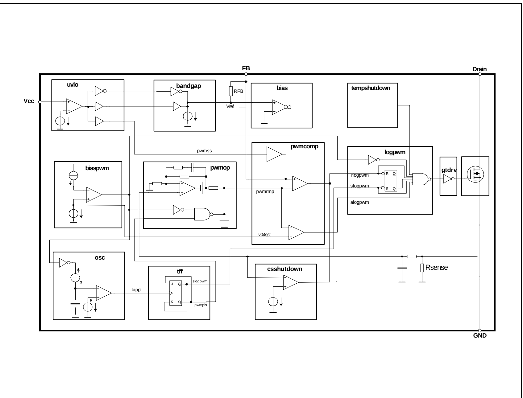
Figure 3 Block Diagram
