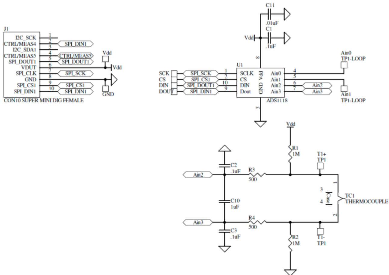
Figure 23. ADS1118EVM Schematic
