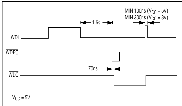
Figure 7. WDI, WDO, and WDPO Timing Diagram
