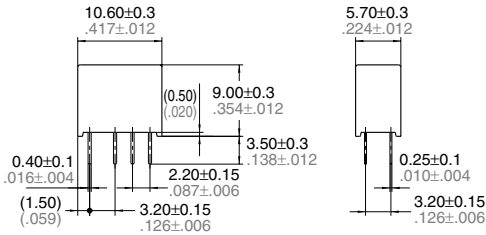
External dimensions Standard type
