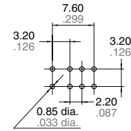
PC board pattern
