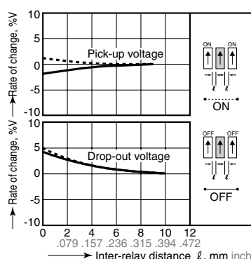
9-(1). Influence of adjacent mounting Tested sample: AGN20012, 6 pcs.
