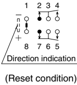
1 coil latching
