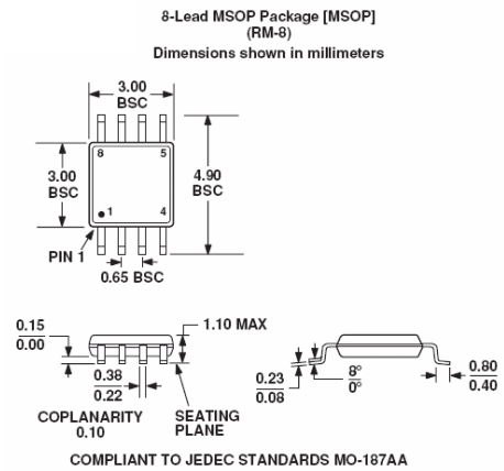
Figure 2. \mu SOIC-8—Dimensions shown in millimeters
