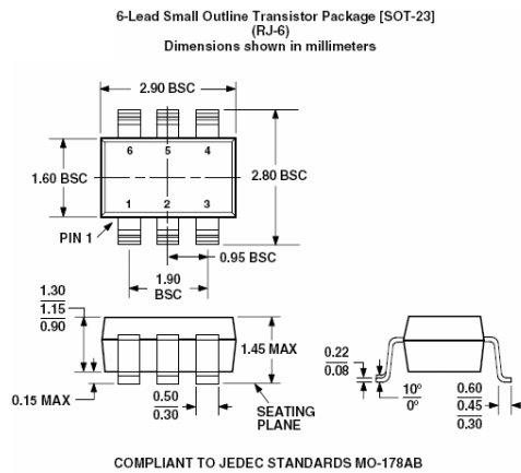
Figure 1. SOT23-6—Dimensions shown in millimeters
