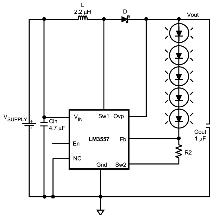
FIGURE 1. Backlight Configuration
