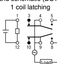
Pin layout and schematic (BOTTOM VIEW)
