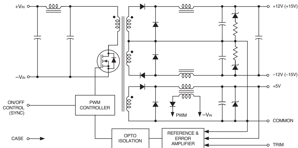
Figure 1. Simplified Schematic
