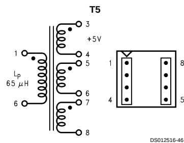
Top View FIGURE 26. Renco RL-5532
