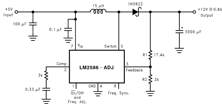
FIGURE 42. Boost Regulator
