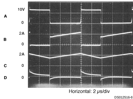
FIGURE 31. Switching Waveforms
