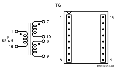
Top View FIGURE 22. Pulse PE-68414 (Surface Mount)
