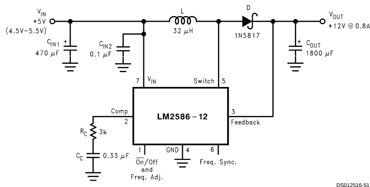
FIGURE 30. 12V Boost Regulator
