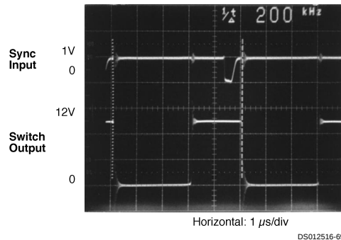
FIGURE 41. Waveforms of a Synchronized 12V Boost Regulator
