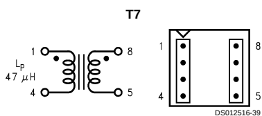
Top View FIGURE 21. Pulse PE-68482
