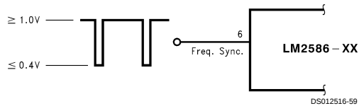
FIGURE 40. Frequency Synchronization
