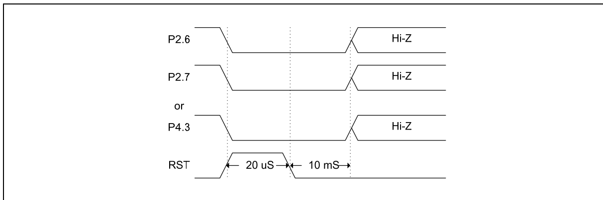
Figure 19-1 Timing of Entering Re-Boot Mode
