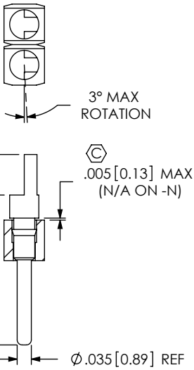
FIG 9 TERMINAL STYLE -C-2 UNLESS OTHERWISE SHOWN, SAME AS FIG1
