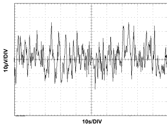
FIGURE 28. V_{OUT} NOISE
