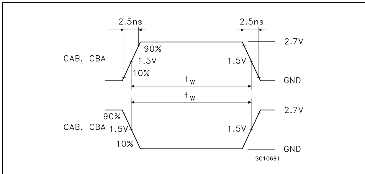
WAVEFORM 4 : PULSE WIDTH ( f=1\text{MHz} ; 50% duty cycle)
