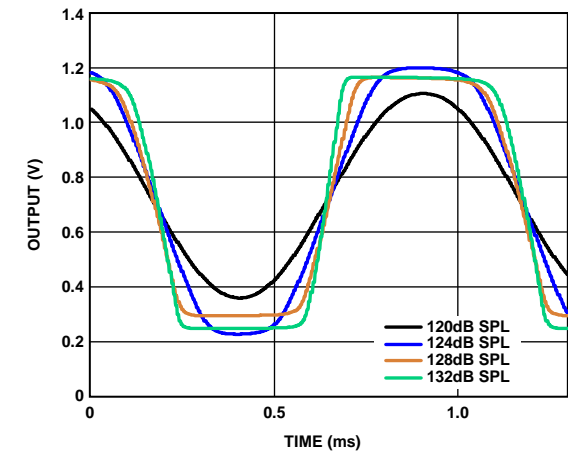
Figure 8. Clipping Characteristics
