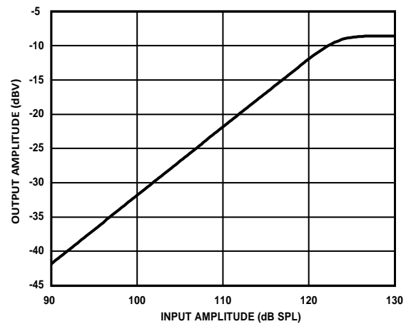
Figure 7. Linearity
