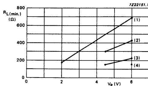
Fig.10 Minimum resistive load as a function of the pull-up voltage.
