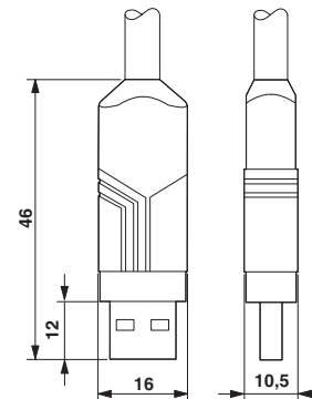
USB plug-in connector, type A, Standard
