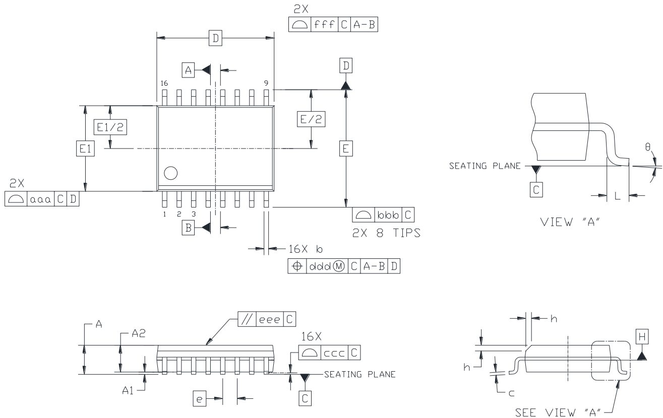
Figure 17. 16-Pin Wide Body SOIC
