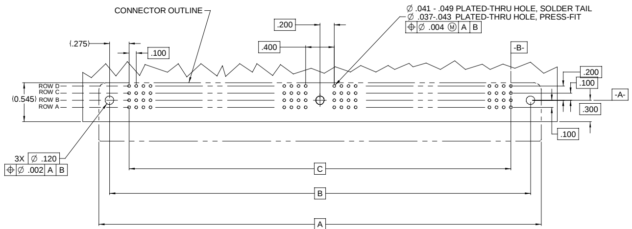
RECOMMENDED P.C.B. HOLE PATTERN
