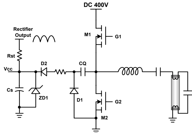
Figure 10. Start-up Circuit
