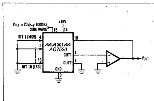
Figure 8. Feedthrough Error
