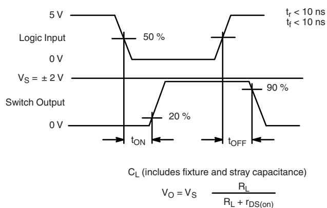
Figure 2. Switching Time
