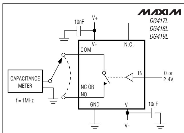
Figure 8. Channel On-Capacitance
