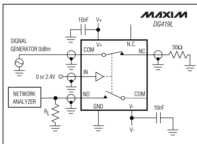
Figure 6. DG419L Crosstalk
