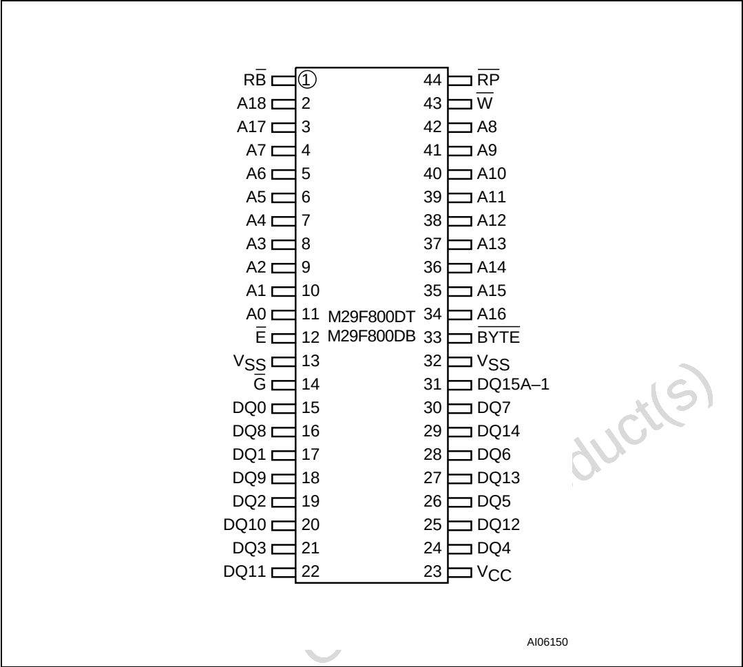
Figure 2. SO connections
