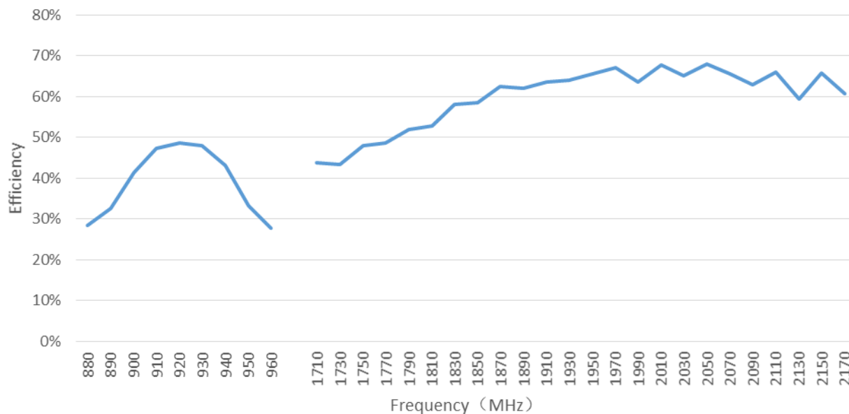
Version 2: Typical free Space Total Efficiencies [%]
