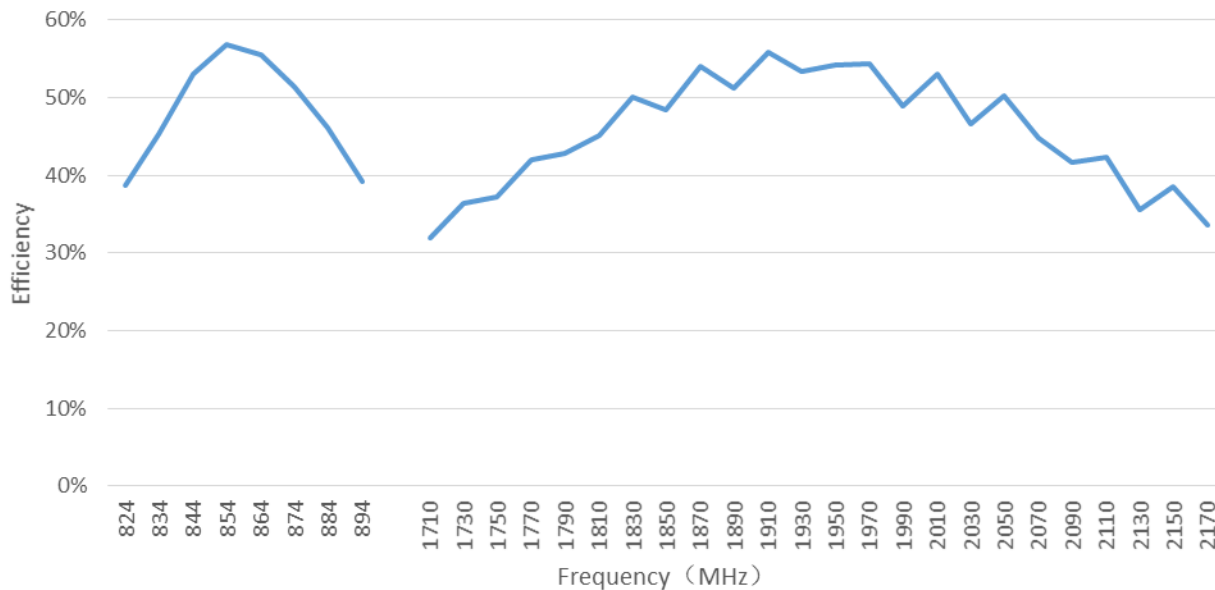
Version 1: Typical free Space Total Efficiencies [%]
