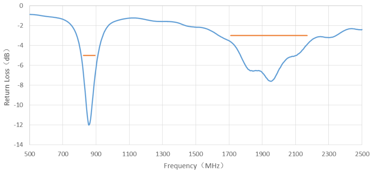
Version 1: Typical Return Loss
