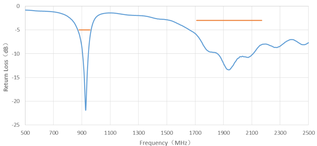
Version 2: Typical Return Loss
