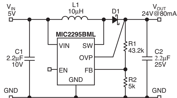
5V IN to 24V OUT @ 80mA
