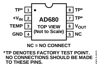
Figure 1. 8-Lead PDIP and 8-Lead SOIC Pin Configuration
