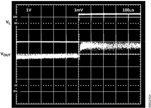
Figure 14. Typical Load Regulation Characteristics
