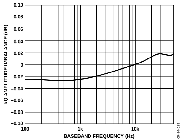
Figure 20. Quadrature (I/Q) Amplitude Error vs. Baseband Frequency
