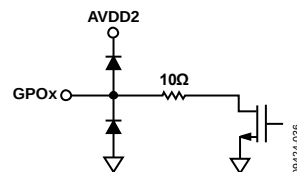
Figure 36. Equivalent GPOx Output Circuit
