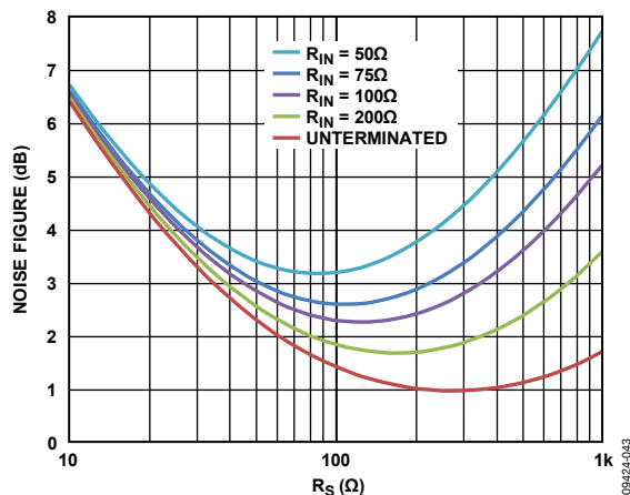
Figure 46. Noise Figure vs. R_S for Various Fixed Values of R_{IN} , Active Termination Matched Inputs, V_{GAIN} = 1.6\ \text{V}
