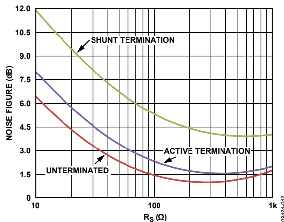
Figure 45. Noise Figure vs. R_S for Shunt Termination, Active Termination Matched and Unterminated Inputs, V_{GAIN} = 1.6\ \text{V}
