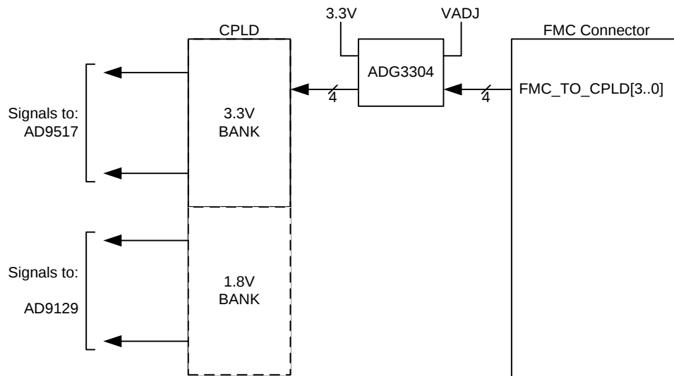
Figure 8: FMC control interface
