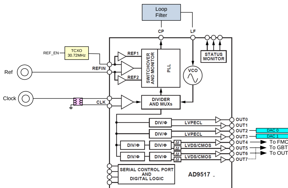
Figure 5: Clock tree
