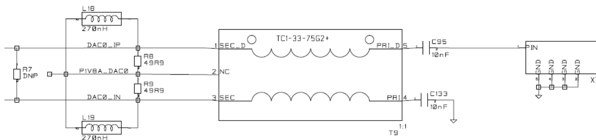
Figure 4: Wideband balun output option
