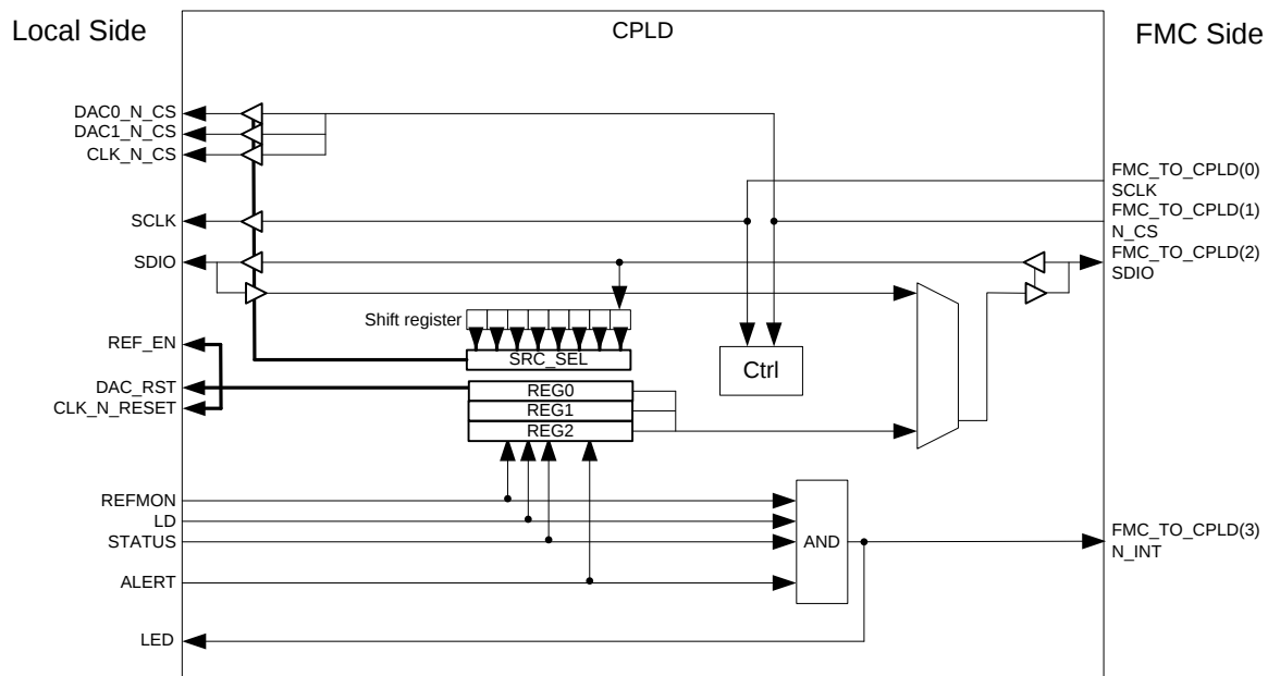
Figure 9: CPLD architecture
