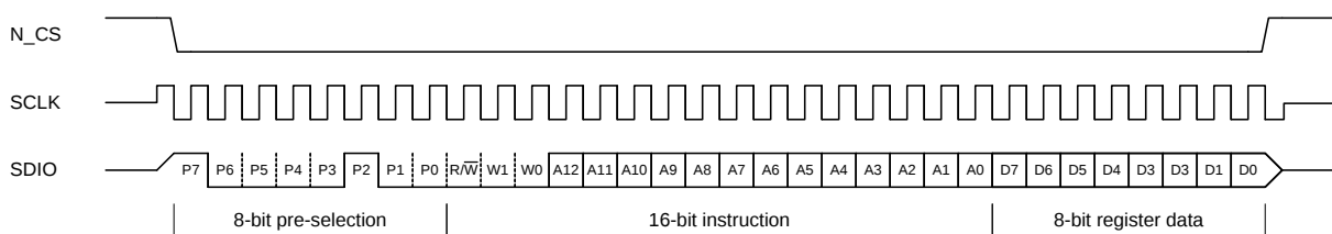
Figure 14: Write instruction to AD9517 registers A12:A0
