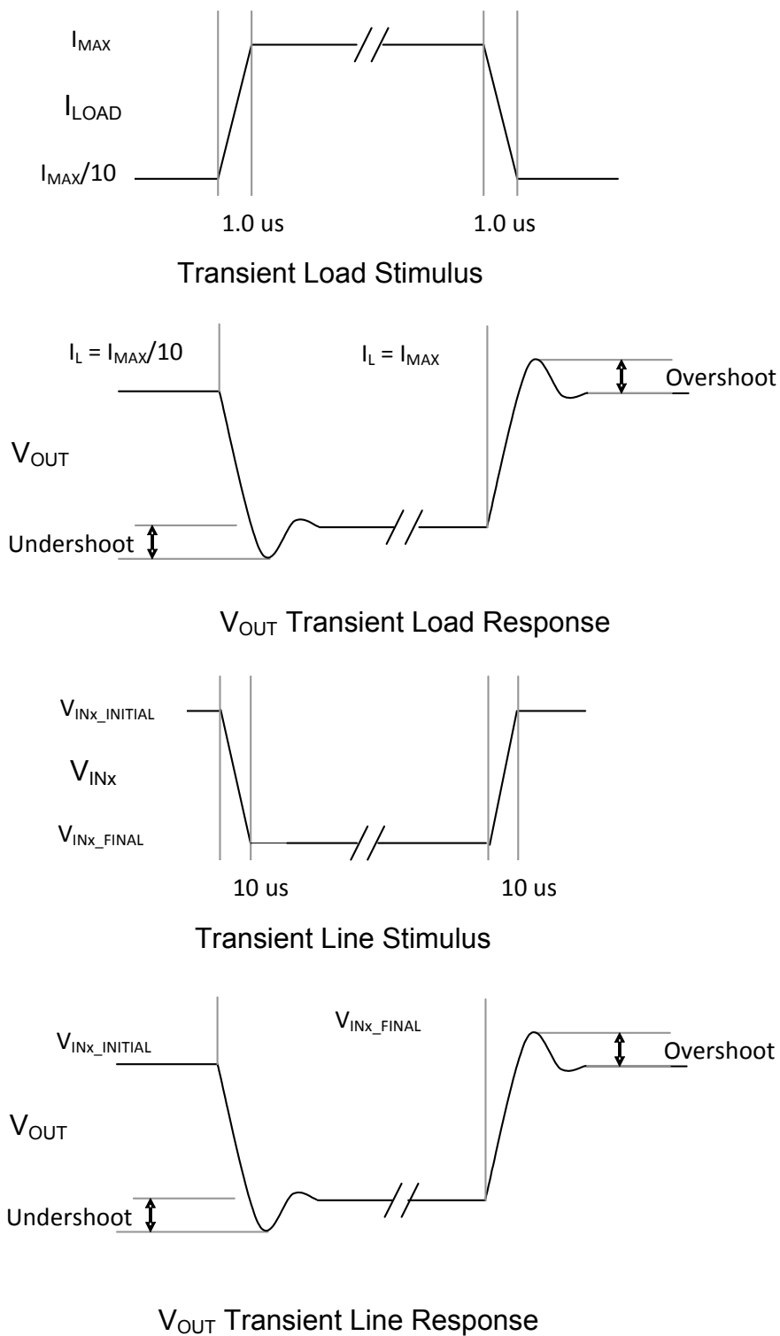
Figure 31. Transient Waveforms
