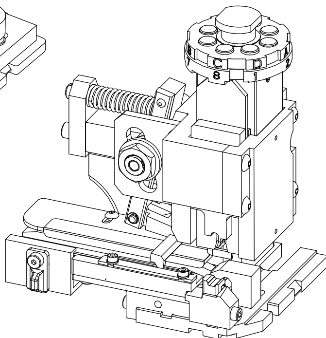
Heavy Duty Industrial (HD-I) Quick-Change Applicator (Side-Feed Type) (Typ)
