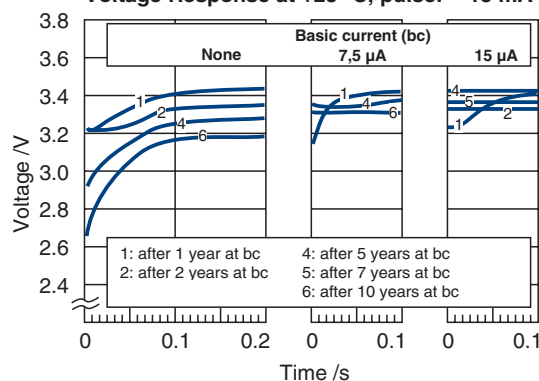
Voltage Response at +25 °C, pulse: 15 mA
