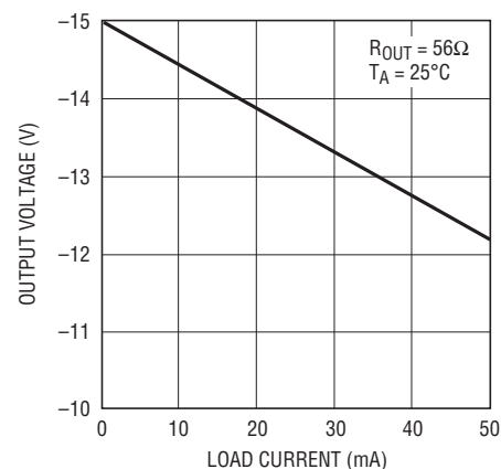
Output Voltage vs Load Current, V^+ = 15\text{V}
