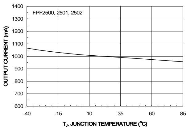
Figure 9. Current Limit vs. Temperature
