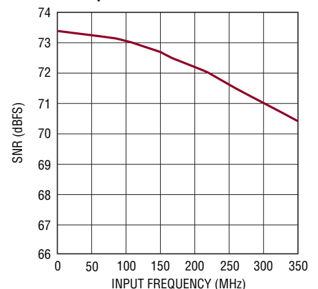
LTC2264-14: SNR vs Input Frequency, -1\text{dBFS} , 2V Range, 40Msps
