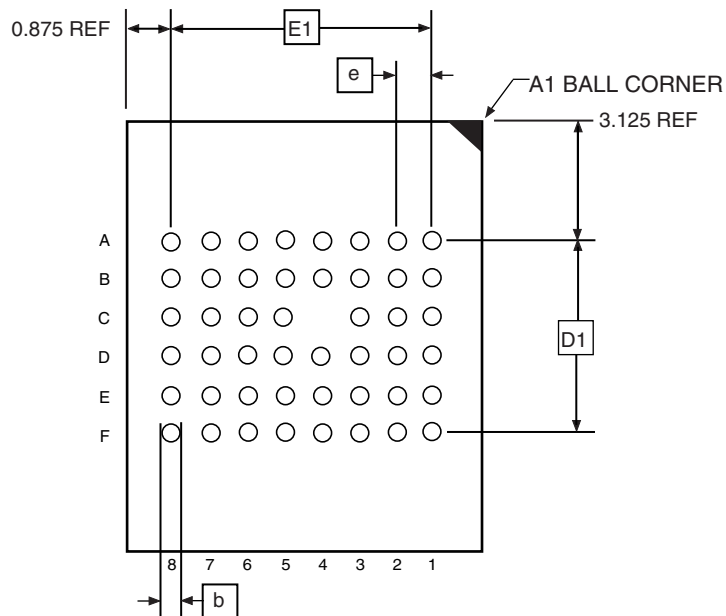
BOTTOM VIEW
