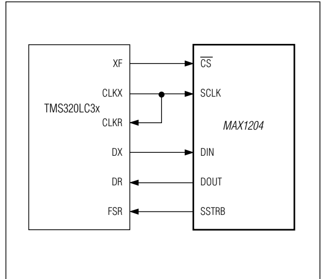
Figure 19. MAX1204 to TMS320 Serial Interface
