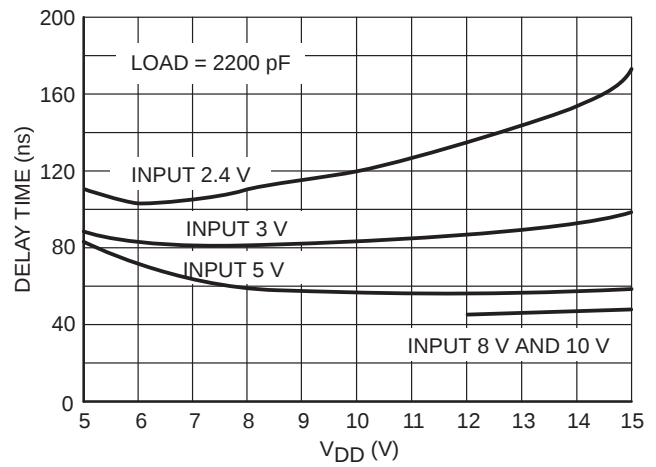
Figure 13. Effect of Input Amplitude on Propagation Delay
