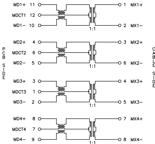
SCHEMATIC
