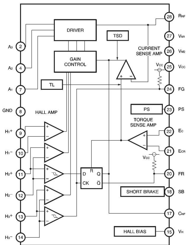
BA6849FP / FM
