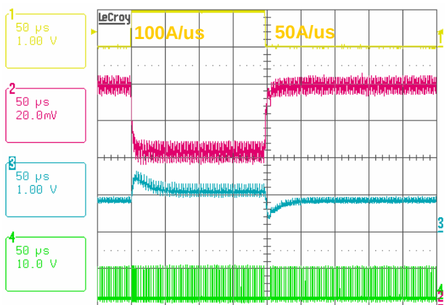
FIGURE 35. LOAD TRANSIENT RESPONSE IN CCM V_{IN} = 8V , I_O = 2A \leftrightarrow 20A , VID = 1.1V, Ch1: Io, Ch2: Vo, Ch3: Vcomp, Ch4: PHASE
