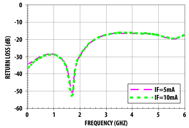
Figure 4. Return Loss vs. Frequency ( P_{in} = 0\text{dBm} )
