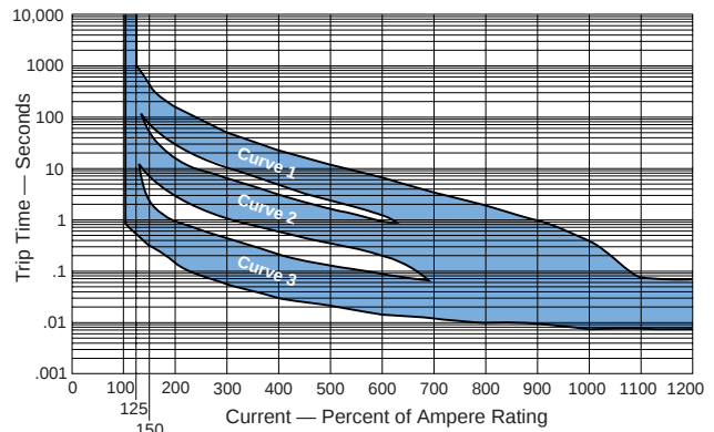
Curves 1, 2 and 3, 50/60 Hz
