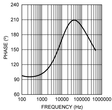
Figure 40. Error Amplifier Phase
