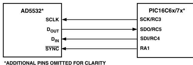
Figure 22. AD5532 to PIC16C6x/7x Interface
