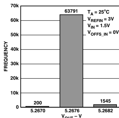
Figure 16. SHA-Mode Repeatability (64K Acquisitions)
