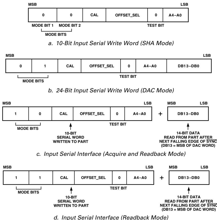
Figure 19. Serial Interface Formats
