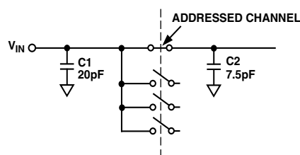
Figure 17. Analog Input Circuit
