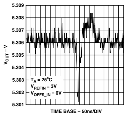
Figure 13. Major Code Transition Glitch Impulse
