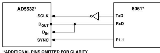
Figure 23. AD5532 to 8051 Interface
