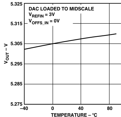
Figure 10. V_{OUT} vs. Temperature
