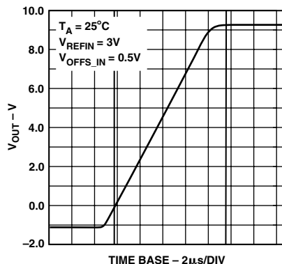
Figure 12. Full-Scale Settling Time
