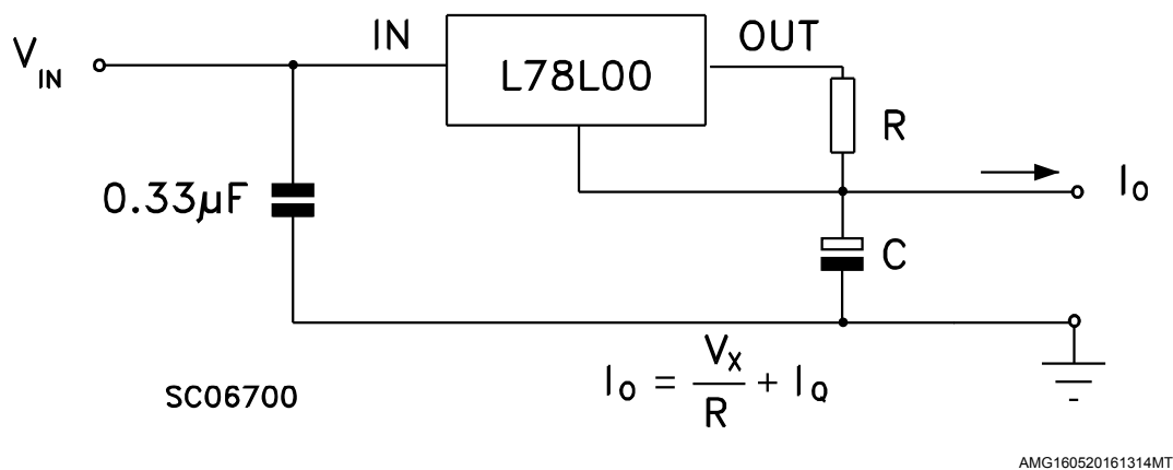
Figure 15. Current regulator
