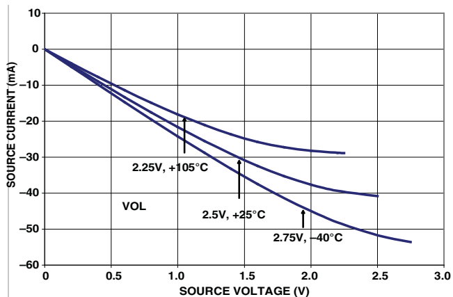
Figure 70. Drive Current E (Low V_{DDEXT} )
