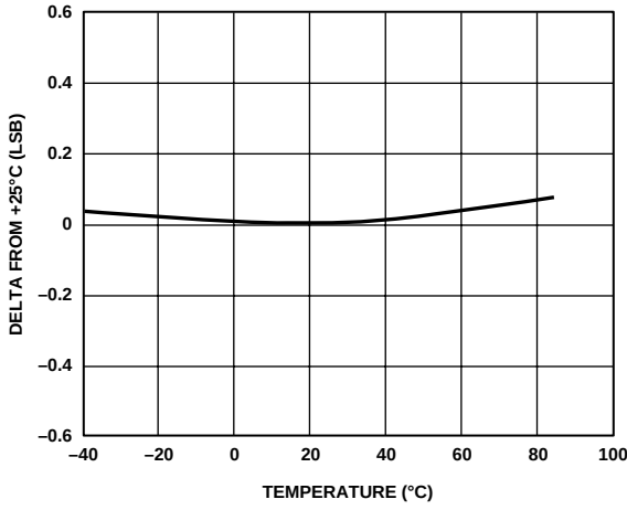
Figure 9. Change in Offset vs. Temperature
