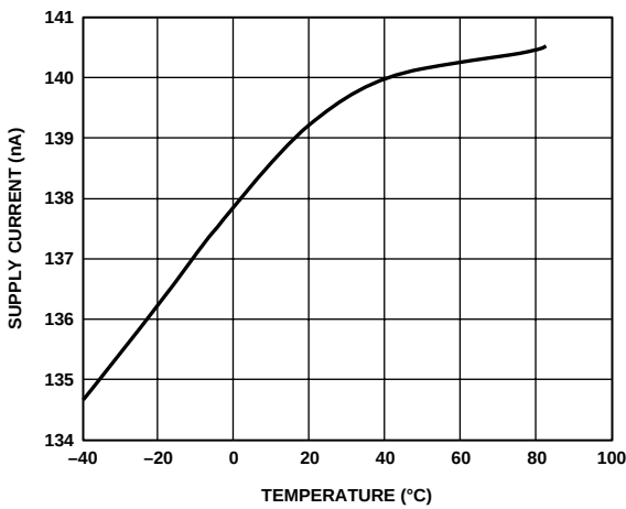
Figure 7. Power-Down Supply Current vs. Temperature
